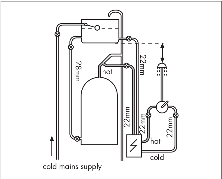
Pumped System
